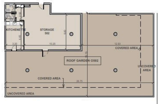
Roof Garden Plan
