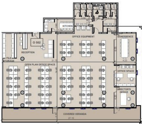
Office Floor Plan
