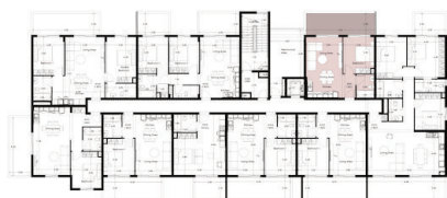
2 nd floor plan
